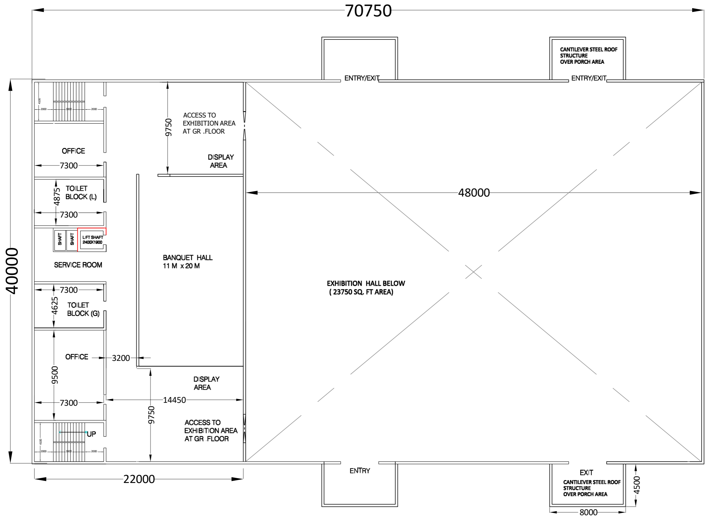
GROUND & FIRST FLOOR PLAN
