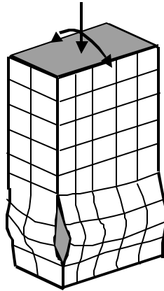
Fig. 10 Failure Mode of a Concrete-filled RHS
