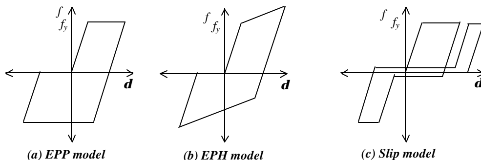
Fig. 5. Hysteretic models
