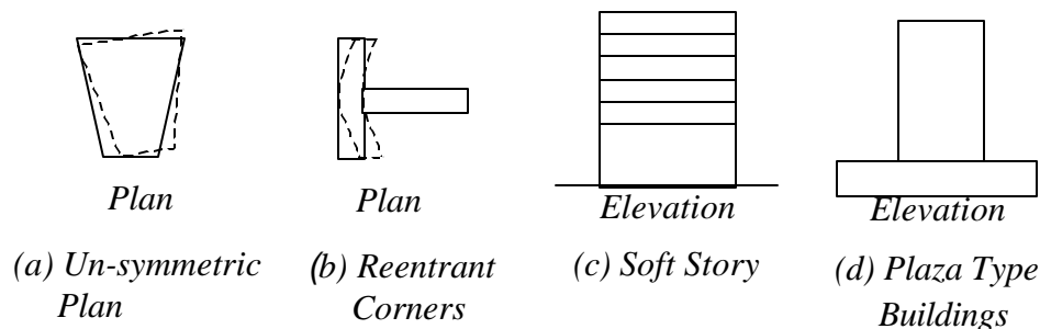
Fig. 2 Irregular Structures
