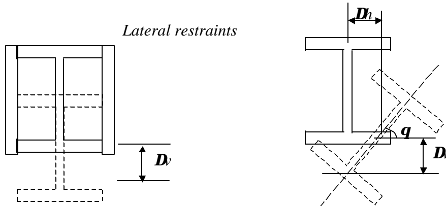
(c) Section at restraint
