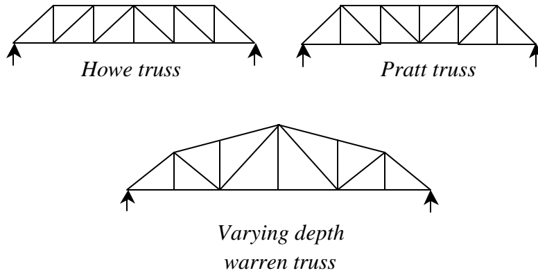
Fig. 2(c) Some of the trusses used in steel bridges
