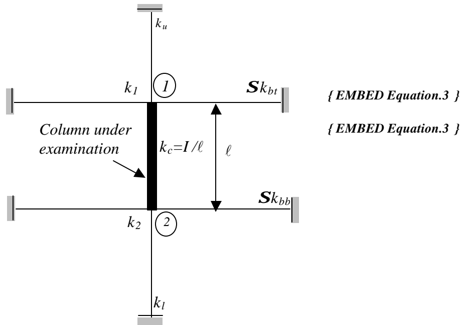
Fig.3 Limited Substitute Frame
