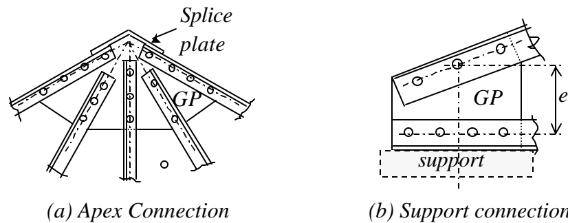
Fig. 7 Truss Connections
