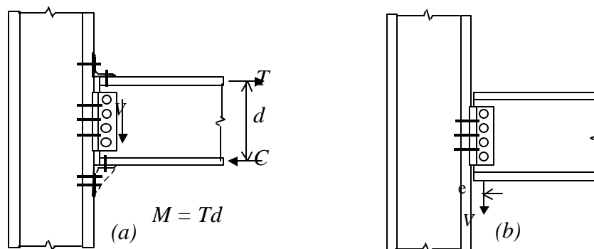
Fig. 1 Standard Connections (a) moment connection (b) simple connection
