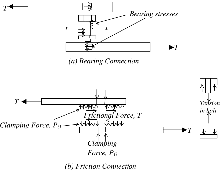
Fig. 7 Bolt Shear Transfer – Free Body Diagram
