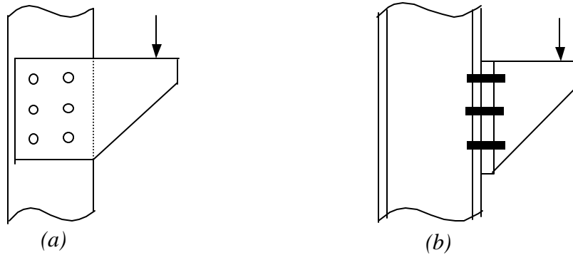
Fig. 2 Moment Connections
