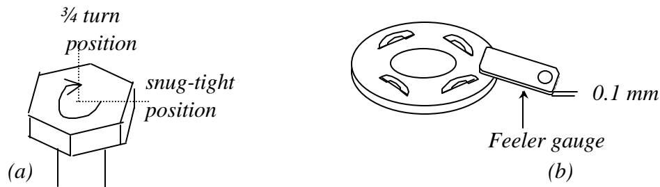
Fig. 5 Tightening of HSFG bolts
