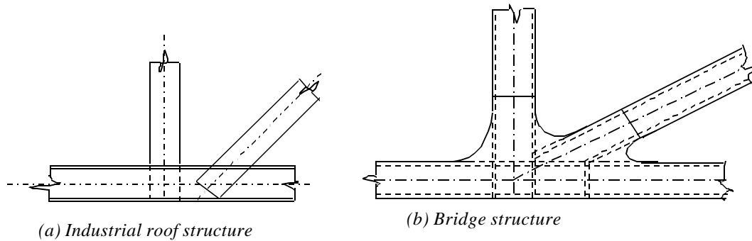
Fig. 3 Typical connection details
