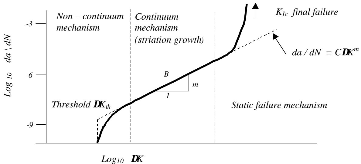
Fig. 11 Schematic representation of crack growth
