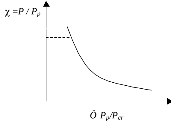
Fig. 4(b) Non-dimensionalised column buckling curve
