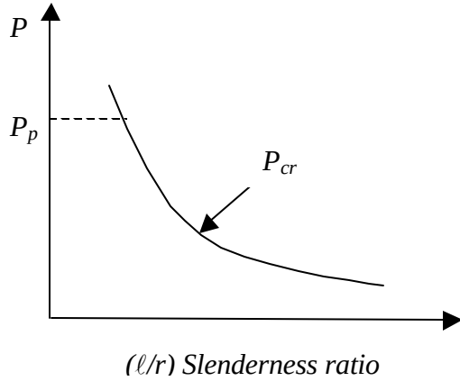
Fig. 4(a): Idealised column buckling curve
