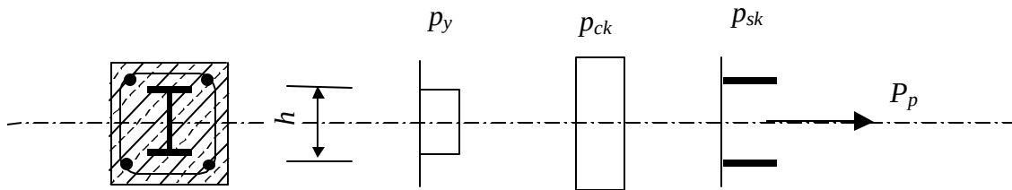
Fig. 3 Stress distribution of the plastic resistance to compression of an encased I section
