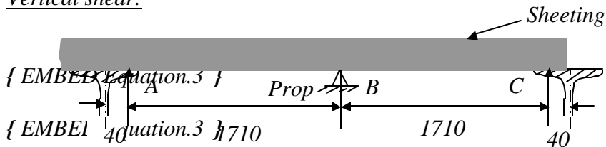
Fig.A2 Profiled sheeting during construction
