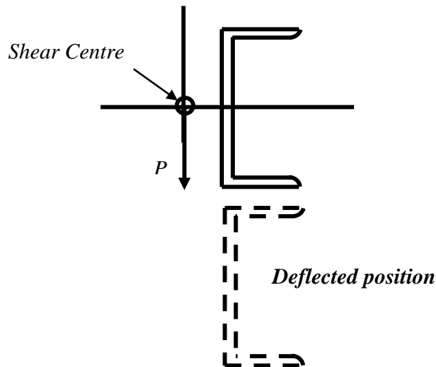
Fig.19 Deflection of channel beam loaded through the shear centre
