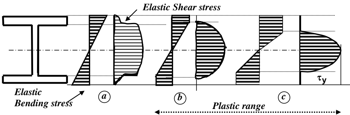
Fig. 8 Combined bending and shear in beams
