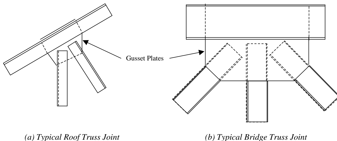
Fig. 6 Typical Truss Joints
