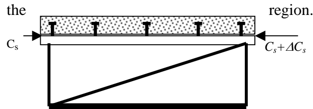
(a) Due to Composite Truss
